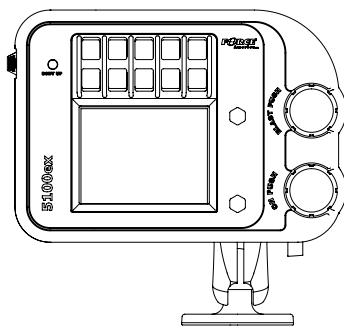
5100ex CONTROLLER
